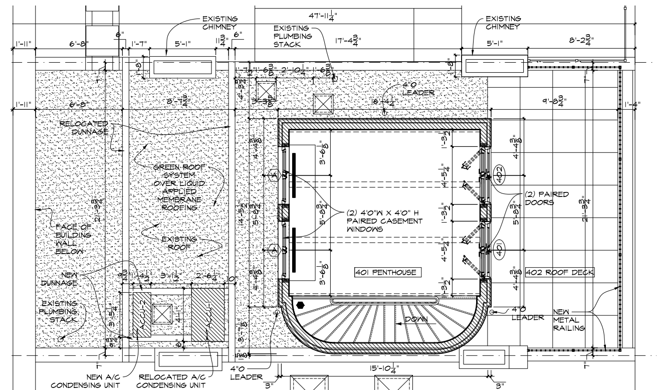
186 Sullivan Street - Proposed Roof Plan
