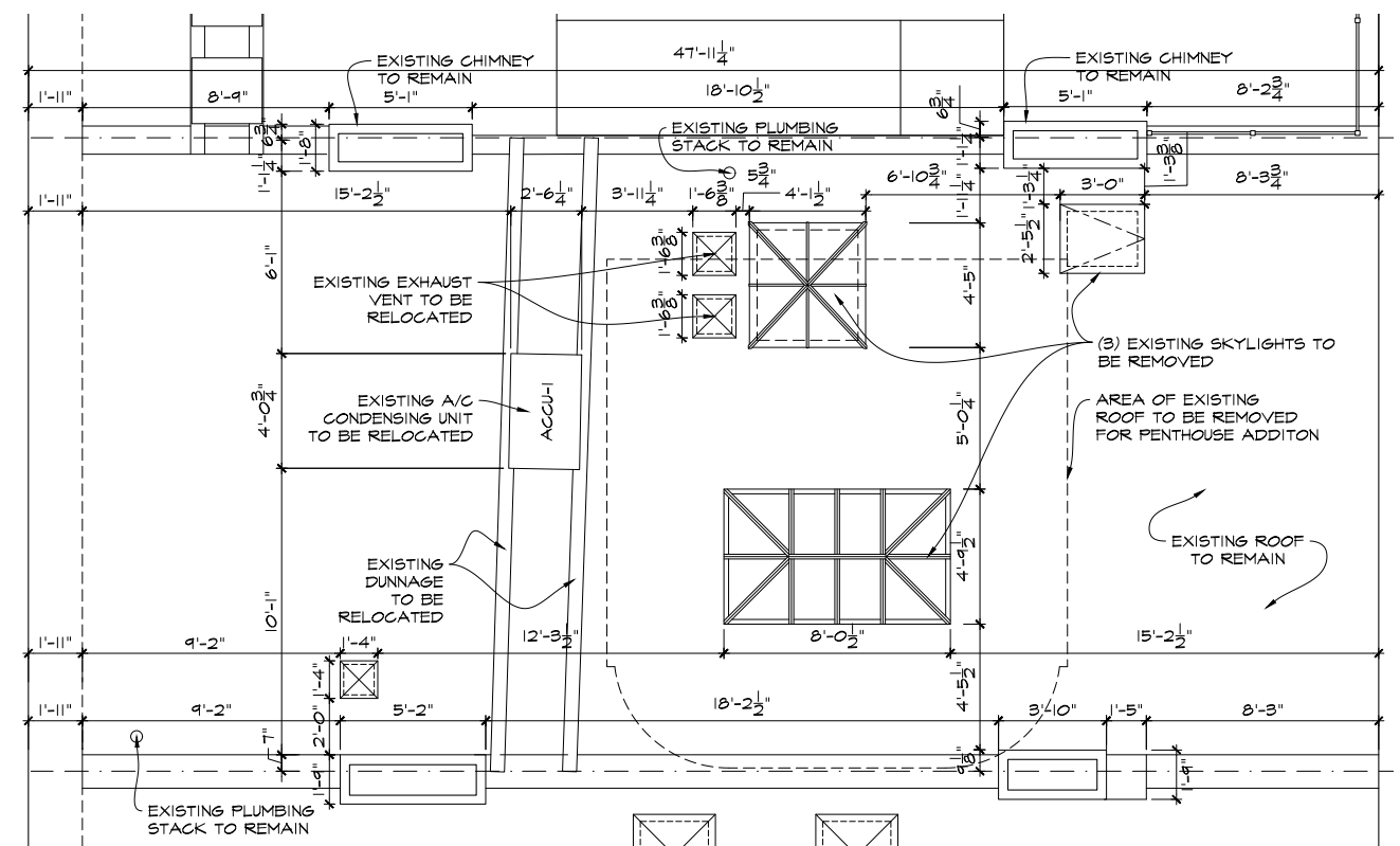
186 Sullivan Street - Existing Roof Plan
