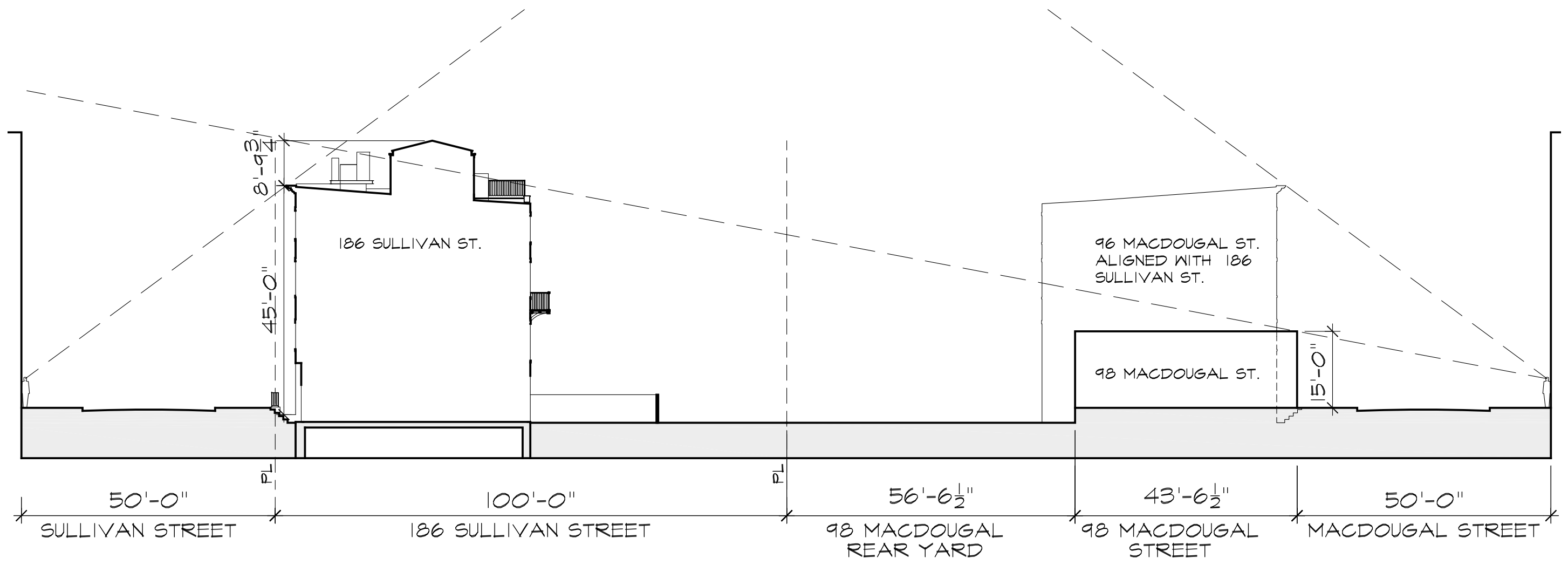
Sight-line Section - Sullivan Street to MacDougal Street
